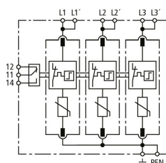
Basic circuit diagram DG MP TNC 150 FM
