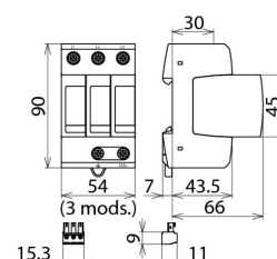
Dimension drawing DG MP TNC 150 FM
