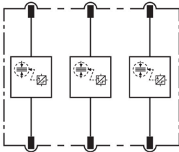
Basic circuit diagram DSE MOD NG 2P 60
