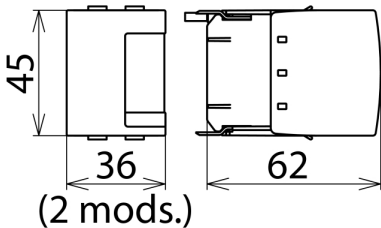
Dimension drawing DSE MOD NG 2P 60
