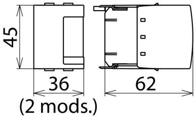
Dimension drawing DB M MOD 150
