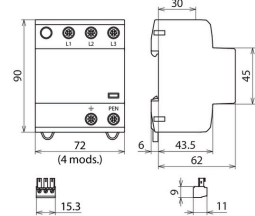
Dimension drawing DSH B TNC 255 FM
