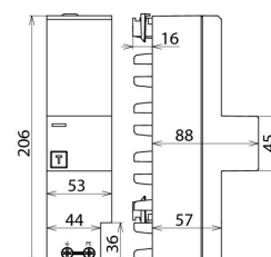
Dimension drawing DV ZP TT 255
