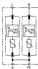
Basic circuit diagram DG M TN 275
